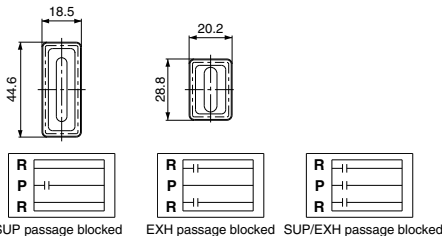
SUP passage blocked
