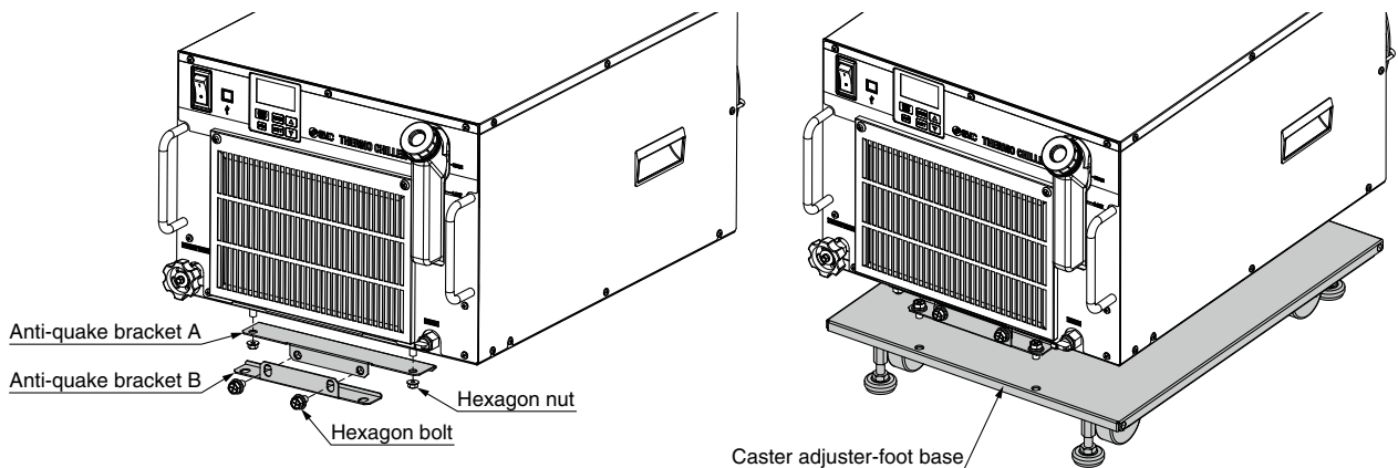
Mounting view
