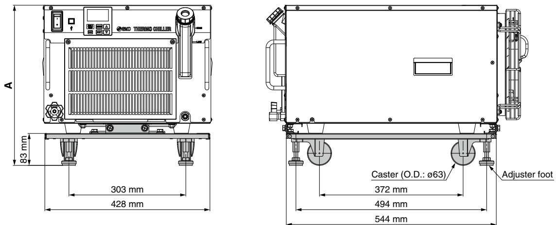
Mounting view (HRR012/018-A-□)
