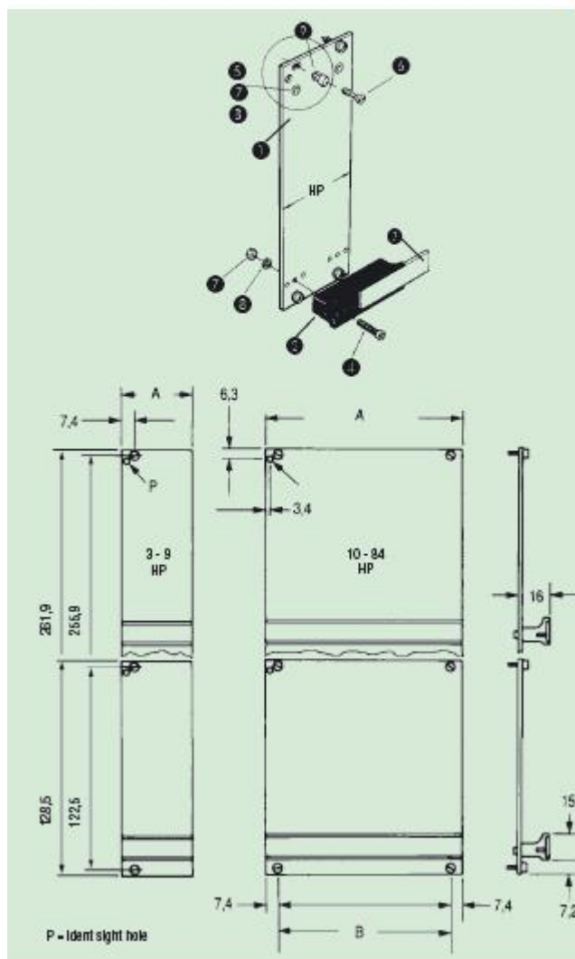
Standard 3U & 6U front panels
