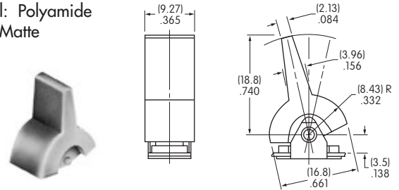
E AT4149 .365" (9.27mm) Wide Paddle
