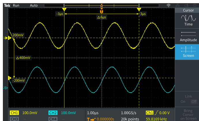
Figure 2: The cursor readouts are presented on the waveform display. Cursors can be used to measure time and amplitude.
