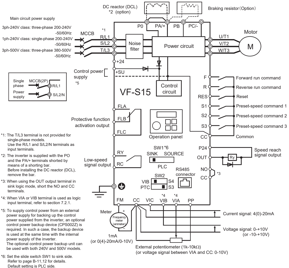
Standard connection diagram - SINK (Negative) (common:CC)
