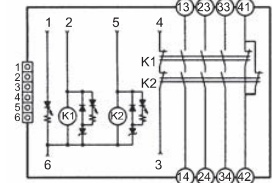
G9SA-EX031-T□
