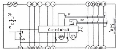
G9SA-TH301 (24 VAC/VDC)
