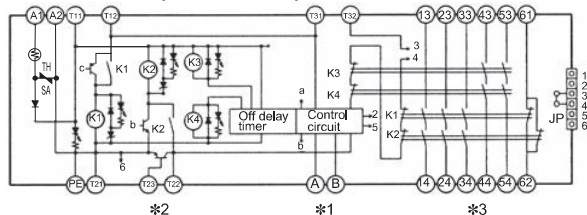
G9SA-TH301 (24 VAC/VDC)
