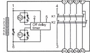
G9SA-EX031-T□
