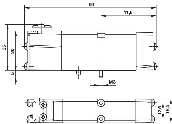
V415537A-X0090 5/2 Single air pilot valve
