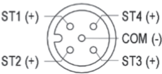
Wiring Diagram
