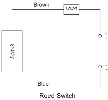
Reed Switch
