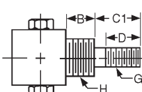
Threaded Nose (NS) Std. on all 1 1/8" bore mounts 1-1/8", 1-1/2" & 2" bores only
