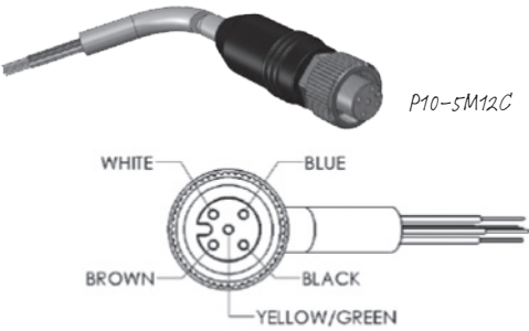
10m M12 Cable
