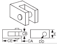
2" & 3" bores
