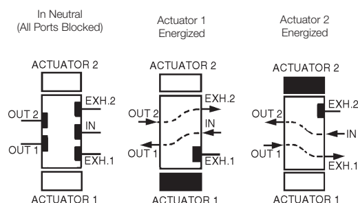
Pressure Held Type (H Models)
