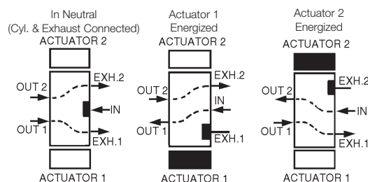
Pressure Release Type (R Models)
