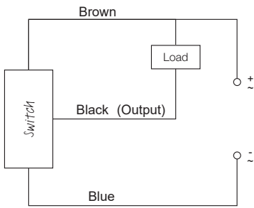
Solid State: Sinking (NPN) Output
