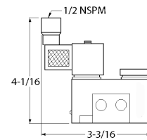
N1-SCD & N2-SCD (with connector)
