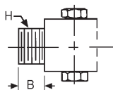
Flush Rear (FR) 1-1/8" bore only
