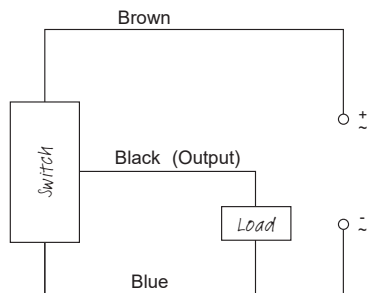
Solid State: Sourcing (PNP) Output
