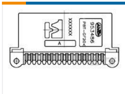
TE Part #953486-1 32pos MQS .63 header 90deg
