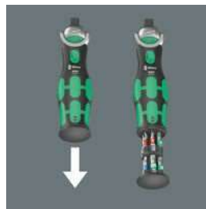
A captive, freely swivelling bit magazine for 12 bits (1/4", 25 mm length) is integrated in the handle of the compact ratchet.
