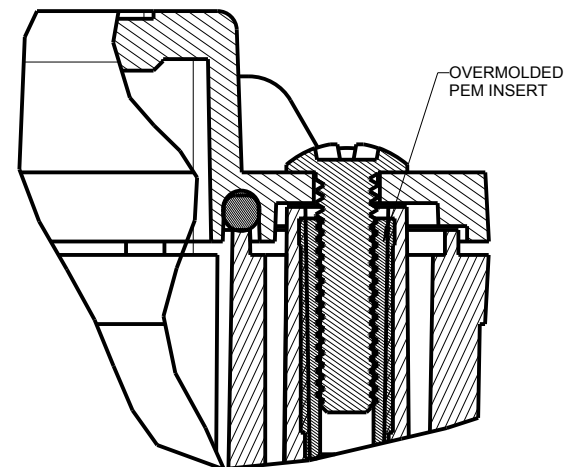
DETAIL D SCALE 2.000
