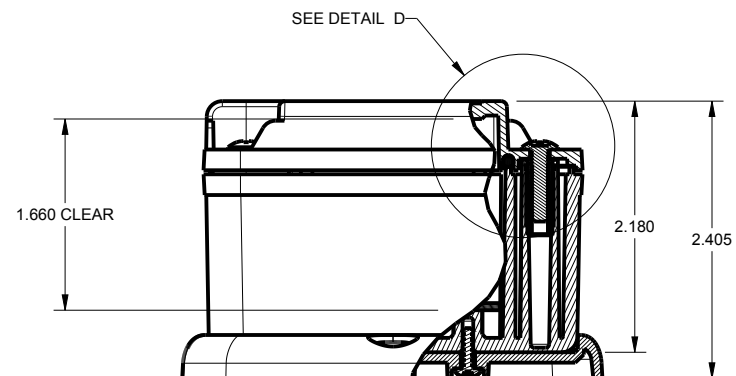
SECTION H-H
