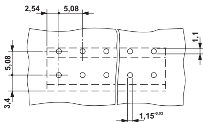
Drilling diagram
