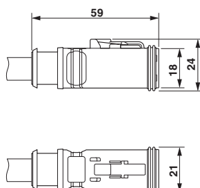
DEUTSCH DT06-3S, top view and side view
