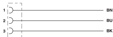
Contact assignment of the DEUTSCH DT06-3S
