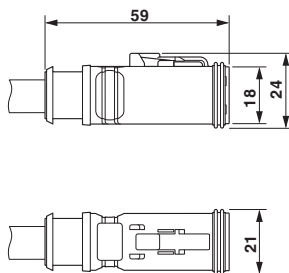
DEUTSCH DT06-3S, top view and side view
