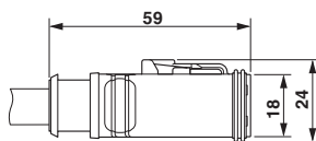
Dimensional drawing
