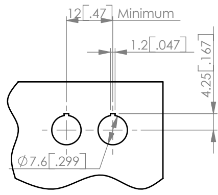
PANEL DETAILS:
