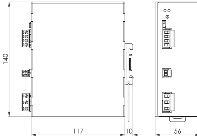
Figure 1. Mechanical Drawing
