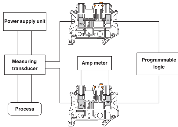
Application drawing
