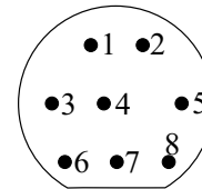
Pin Configuration View A-A (Solder Side)
