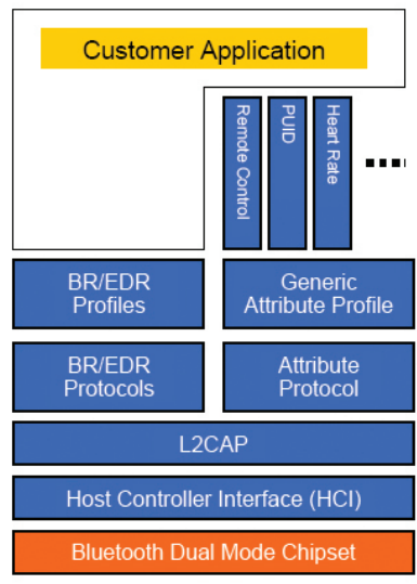
Dual Mode Bluetooth Architecture
