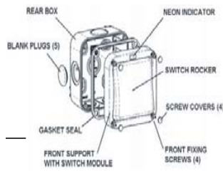
1 gang switch - exploded view
