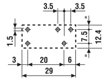
Copper side view Pin length 5.3 mm for PCB or sockets
