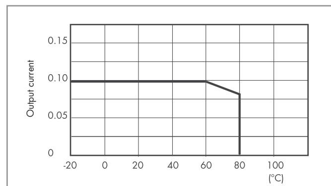
L 34 - Output current v ambient temperature SSR - 0.1 A DC output types
