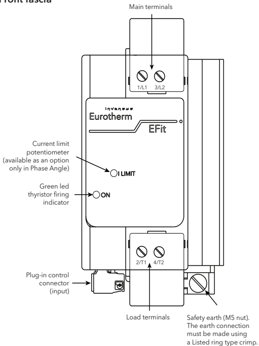
FRONT FASCIA
