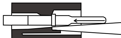
SCREW DRIVER INSERTED TO UNLOCK CONTACT
