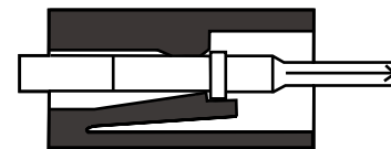
CONTACT LOCKED IN POSITION
