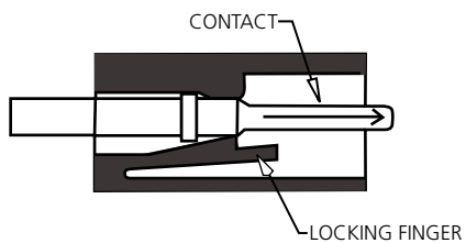
UNLOCKED POSITION
