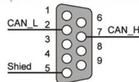
9-pin D-sub male connector
