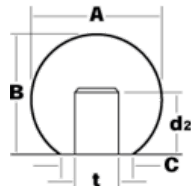
Dimension Chart
