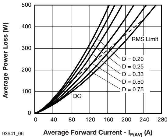
93641_06 Average Forward Current - I F(AV) (A) Fig. 6 - Forward Power Loss Characteristics
