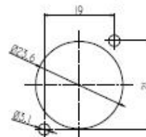
Panel cut out (Rear side)
