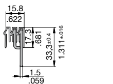
Plug-on cap, busbar 2/3-pole Y 308 506 01
