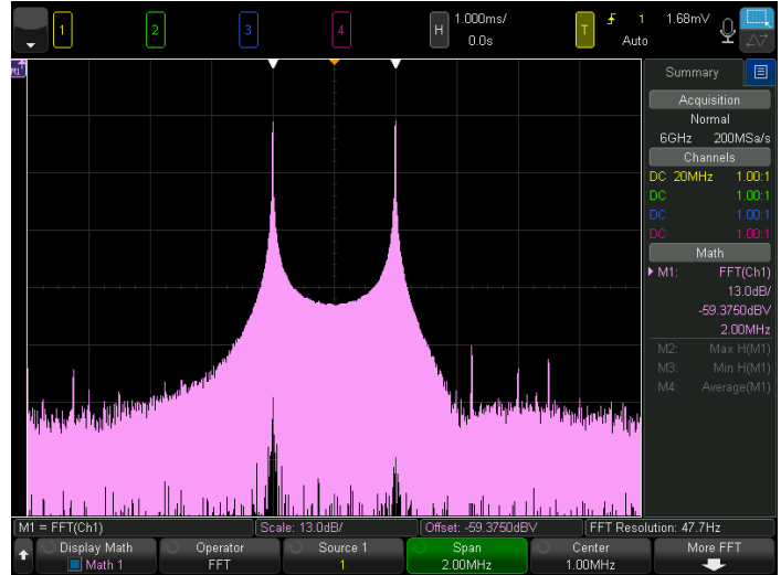
Figure 36. Traditional monochrome FFT with limited features.
