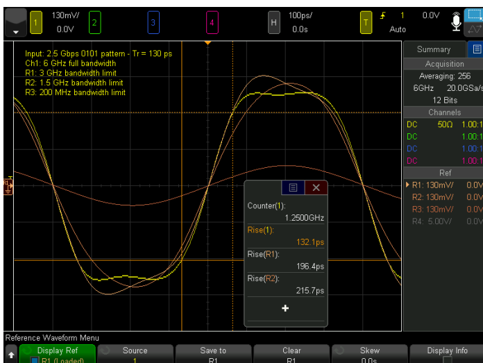
Figure 1. Measuring the rise time of a 130-ps rise-time edge (10-90%). The rise time measurement by – Channel 1 at 6-GHz bandwidth (yellow): 132 ps – Reference 1 (R1) at 3-GHz bandwidth limit: 196 ps – Reference 2 (R2) at 1.5-GHz bandwidth limit: 216 ps
