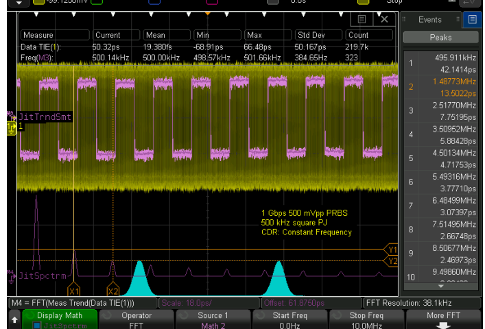
Figure 19. Analyzing periodic jitter (square) on a 1-Gbps PRBS signal.
