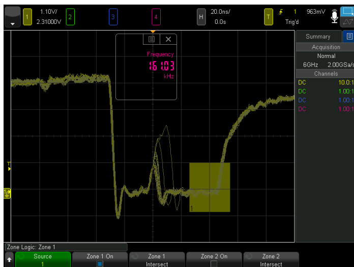
Figure 12. Hardware InfiniiScan Zone triggers immediately.
