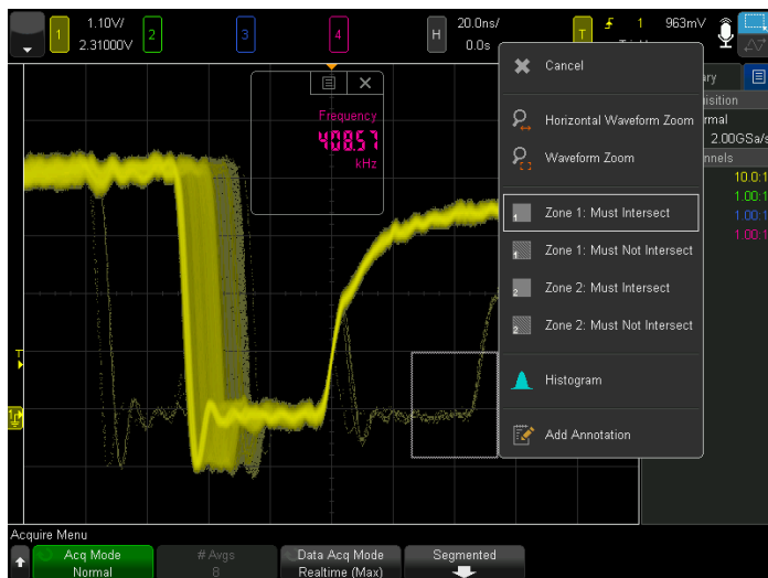
Figure 11. Draw a zone (box) around the anomaly.
