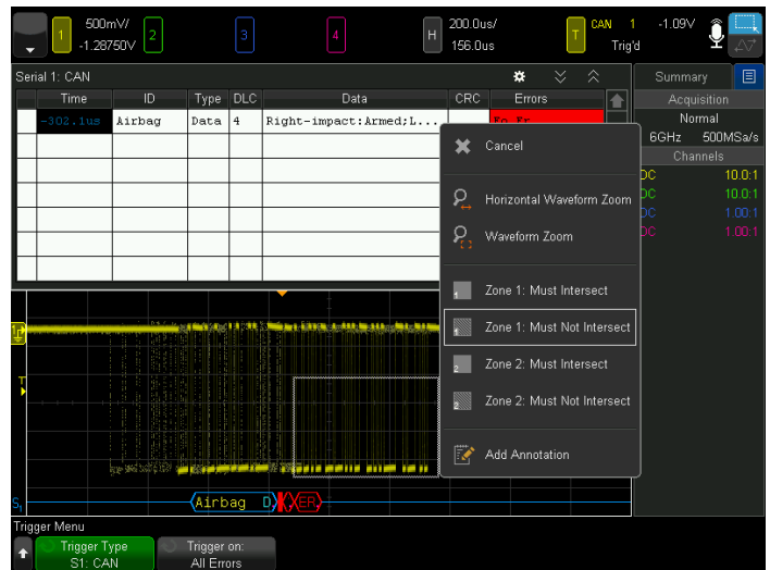
Figure 13. Setting up the InfiniiScan Zone trigger in addition to a CAN bus error packet trigger.
