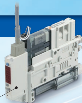
Digital pressure switch for vacuum with energy saving function
