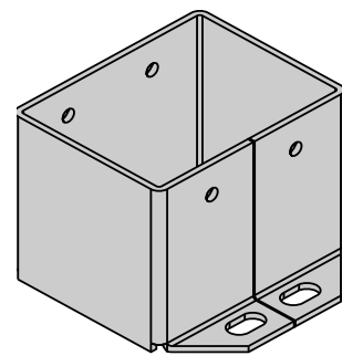
Principle sketch flange steel mounting brackets
