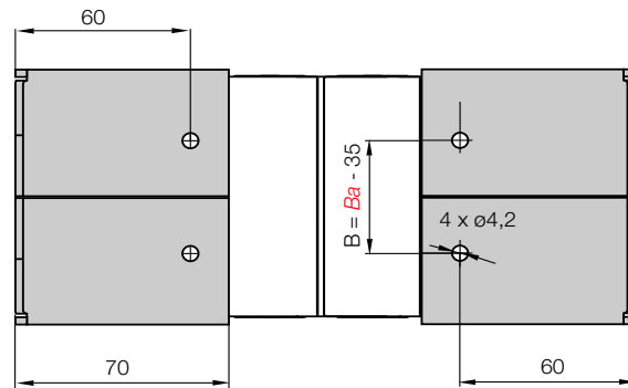
905.050.X Moving end
