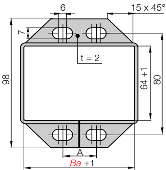
Hole patterns flange steel mounting brackets 905.050.X
