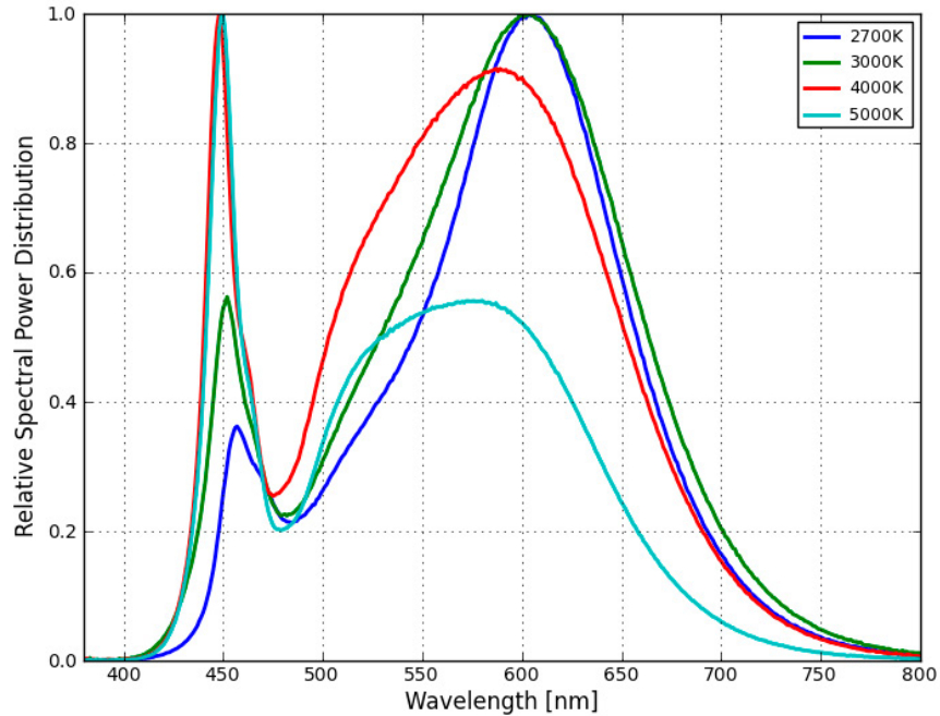
Figure 4. Color spectrum, L130-xx800020102R1 80CRI.
