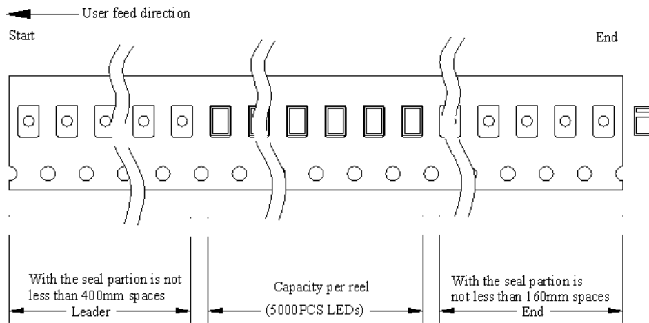
Figure 10. Emitter pocket tape packaging.
