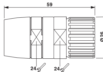
Dimensioned drawing
