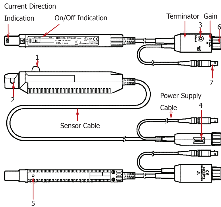
Figure 1 RP1003C Parts
