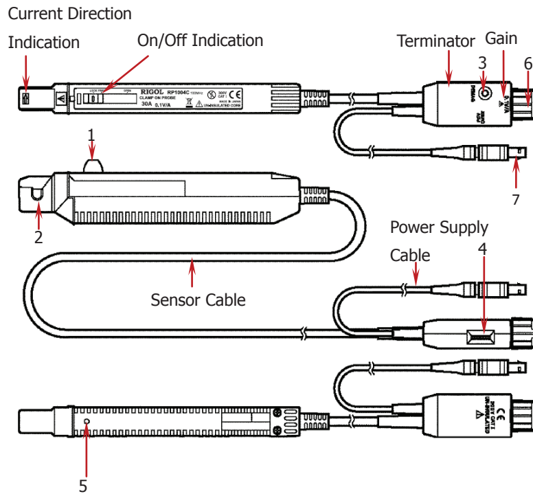
Figure 2 RP1004C Parts
