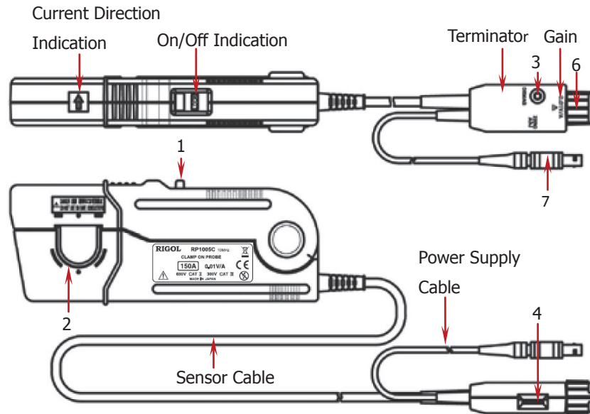
Figure 3 RP1005C Parts
