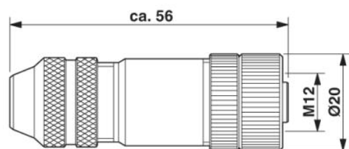
M12 x 1 female connector, straight, shielded
