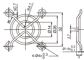
FG-04 For 40mm Fan
