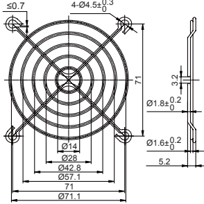
FG-08 For 80mm Fan
