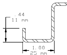
SECTION Z-Z
