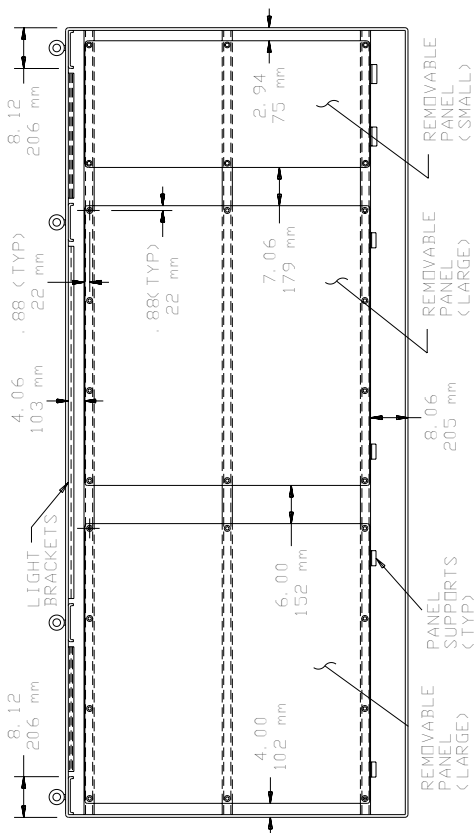
SECTION Y-Y
