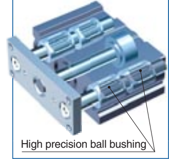
Ball bushing
