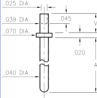
31XX-X-00-XX-00-00-08-0 Swage mount in .043 hole
