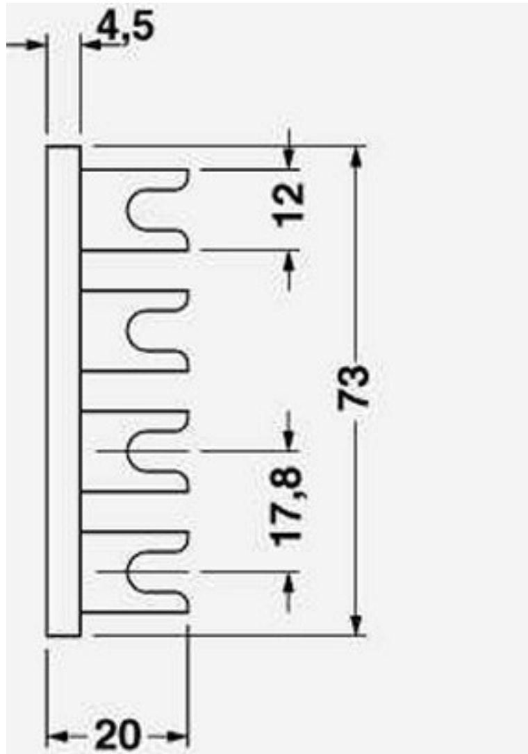
Dimensioned drawing
