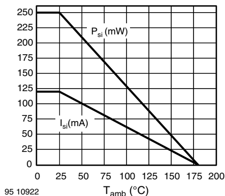
Fig. 1 - Derating Diagram
