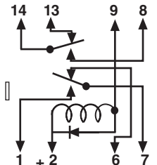
DPDT WITH DIODE
