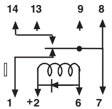
DPDT WITH DIODE
