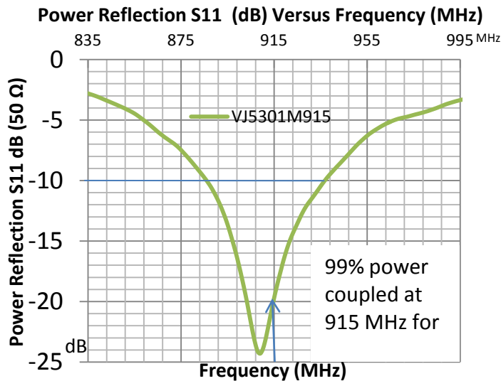
Figure 2 VJ5301M915 tuned to 915 MHz with 99% power coupled
