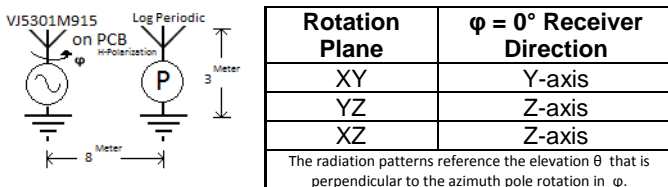
Figure 3 VJ5301M915 PCB mounting and coordinate directions
