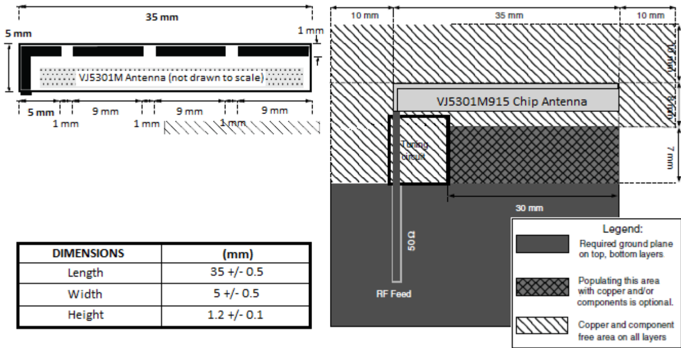
Figure 7 of VJ5301M915 footprint, chip antenna mechanical dimensions, and PCB layout dimensions
