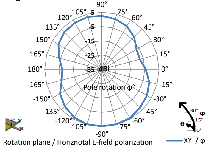
Figure 5 VJ5301M915MXBSR YZ Radiation Pattern
