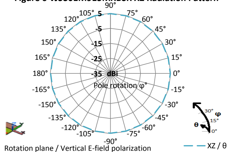
Figure 6 VJ5301M915MXBSR XZ Radiation Pattern
