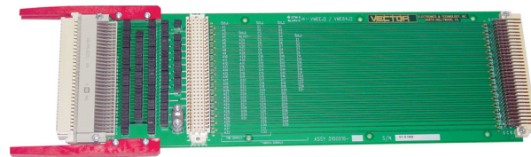
VME64J2 (3U, VME64x J2 w/5-row, 160-pin connector)
