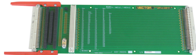
VMEEJ2 (3U, VME J2 w/3-row, 96-pin connector)
