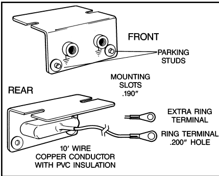
Figure 1. 09740/09741 wrist strap bench ground.
