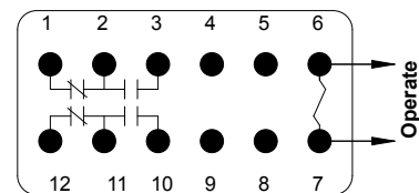
311 Wire Diagram (Top View)
