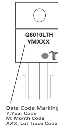
TO-220 AB - (L Package)
